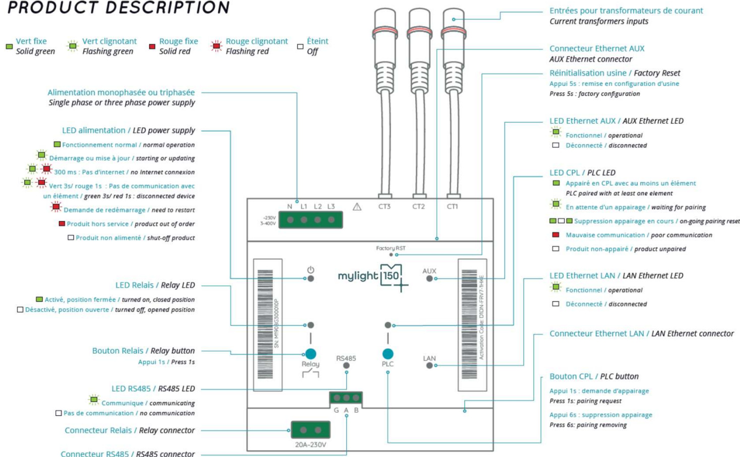
Figure 14. G3Description de la Smart Master
